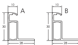
Frame cross section
