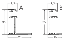
Frame cross section
