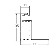
Frame cross section
