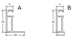
Frame cross section
