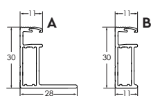
Frame cross section
