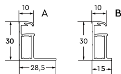
Frame cross section
